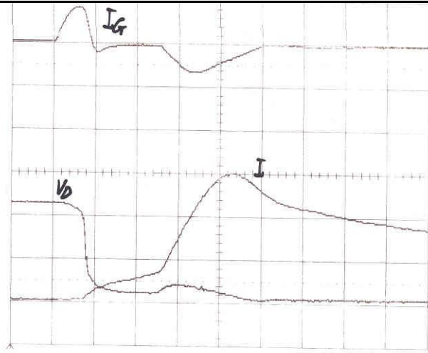
Fig. 12 — Gate current distortion at very high di/dt , t = 2 \mu s/div , I_G = 5 A/div , V_D = 2kV/div , I = 1 kA/div , thyristor 5STP 12N8500 at T = 90^\circ C
