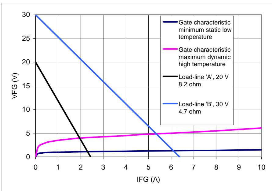
Fig. 7 — Examples of gate-driver load-lines
