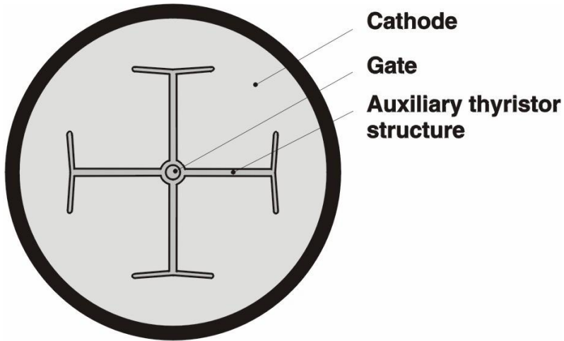
Fig. 4 — View of thyristor wafer with distributed gate (T-Gate)
