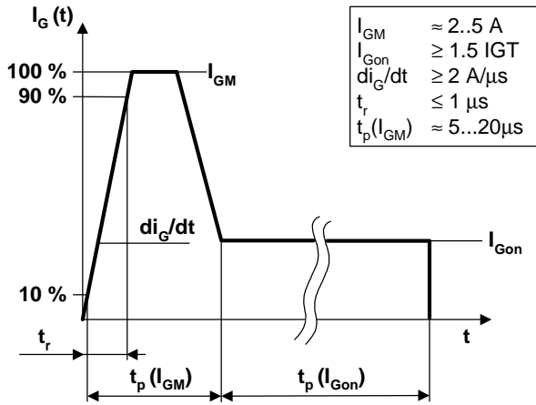
Fig. 6 — Recommended gate-pulse for ABB phase-control thyristors
