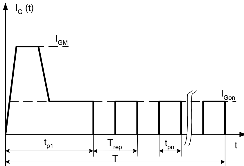
Fig. 9 — Example of a picket-fence gate-pulse train
