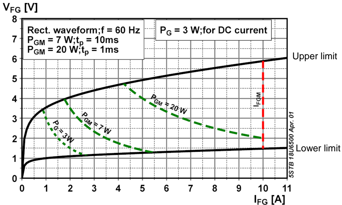
Fig. 1 — Gate characteristic curve from the 5STB 18U6500 data sheet
