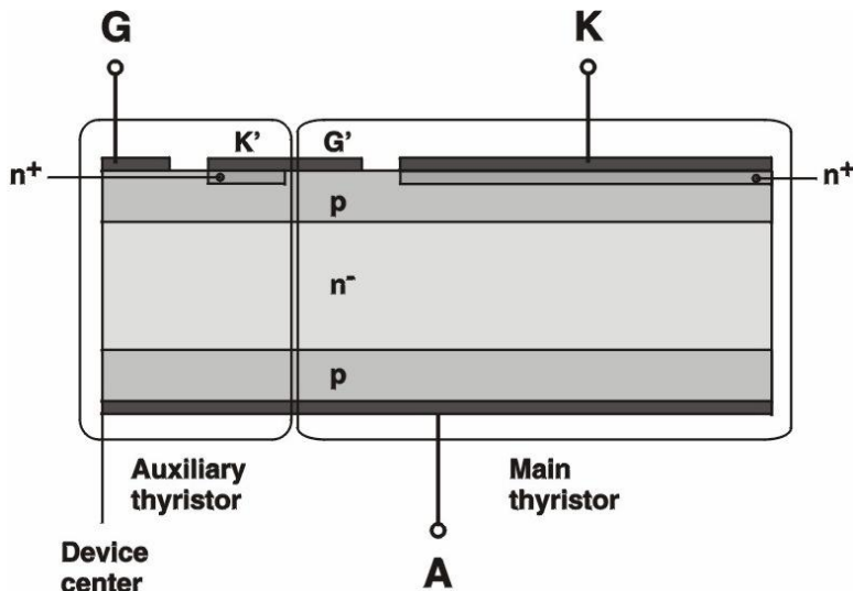
Fig. 3 — Lateral integration of the amplifying gate
