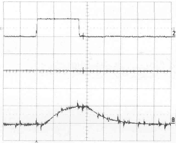
Fig. 10 — Leakage current increase due to gate current for 5STP 25L5200 at V_R = 1500\text{ V} , I_G = 2\text{ A} (channel 2), T_j = 100\text{ }^\circ\text{C} , I_r = 200\text{ mA/div} (channel B), t = 20\text{ }\mu\text{s/div}
