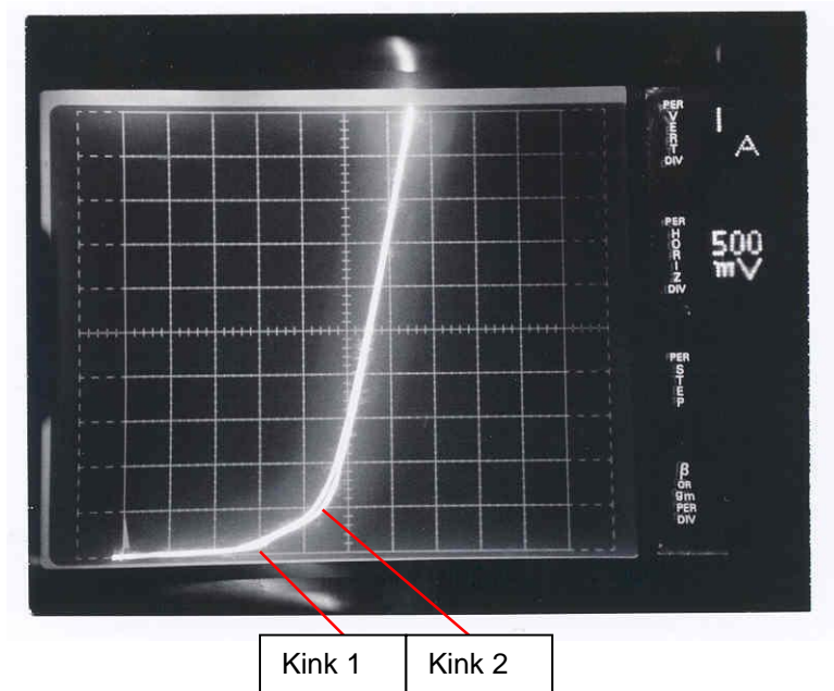
Fig. 5 — Amplifying gate characteristic of thyristor 5STP 26N6500
