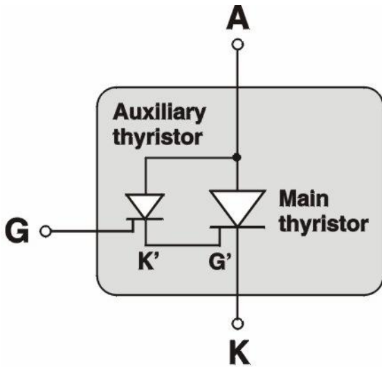
Fig. 2 — Basic principle of the amplifying gate
