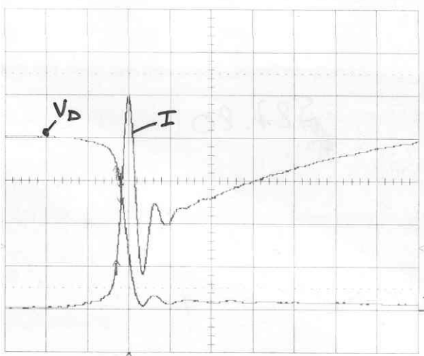
Fig. 8 — Discharge of 20 nF parasitic capacitance using 5STP 25L5200 at V_D = 4000 V, t = 0.5 μs/div, I = 100 A/div, T_j = 90 °C.
