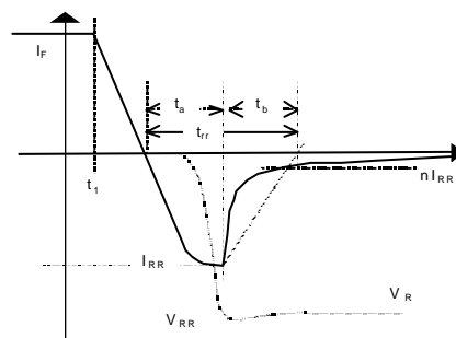
Fig. 2e) Snubberless, clamped induc- tive switching
