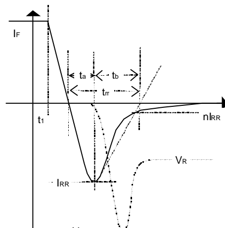
Fig. 1 Soft Recovery and basic parameter definitions
