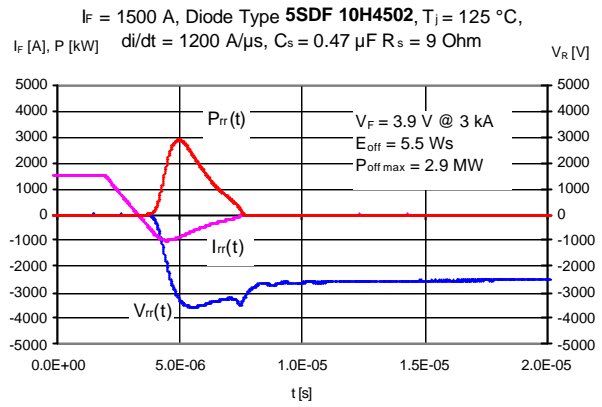
Fig. 8b High resistivity (2.8 kV DC ) at on-set of snap
