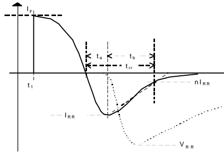
Fig. 2b) R-snubber for RCD, snubber- diode, inductive switching
