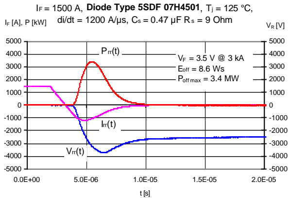
Fig. 8a Low resistivity (2.2 kV DC ), soft recovery
