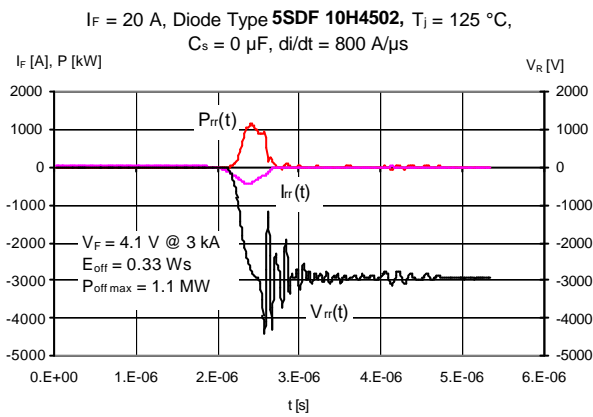
Fig. 7c Poor response of a Category V diode tested as an Undeland snubber (Category III)
