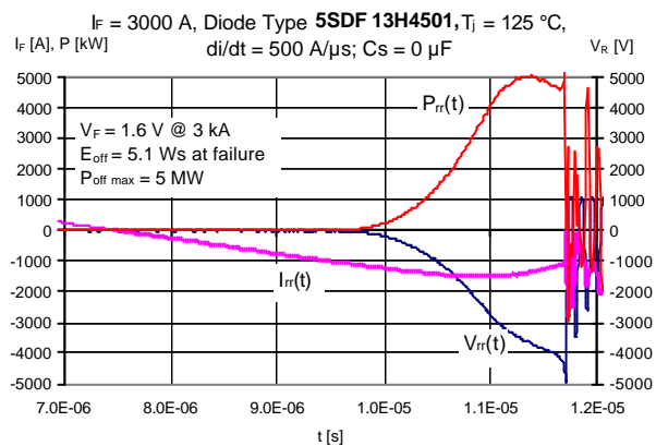
Fig. 9b Uniform life-time FWD at 500 A/μs
