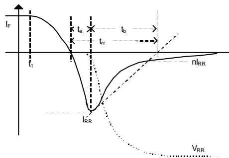
Fig. 2c) Snubberless Undeland/ McMurray snubber-diode, resistive switching
