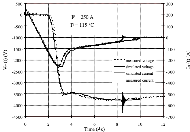
Fig. 10 Measured and simulated recovery of snubberless clamped inductive switching of 6 kV diode type 5SDF 03D6004. (Cat. V diode in Cat. V application)
