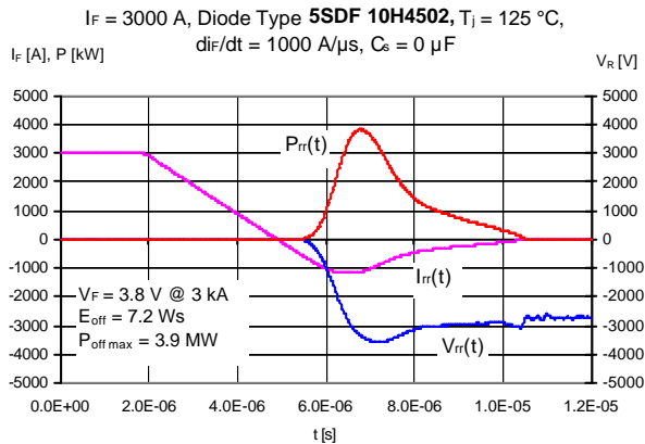
Fig. 9a Profiled life-time FWD at 1000 A/μs
