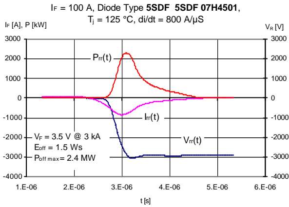
Fig. 7a Undeland snubber diode at “max.” I_F showing soft recovery
