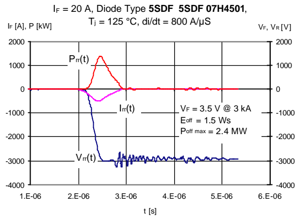
Fig. 7b Undeland snubber diode at “critical min” I_F showing on-set of snap-off
