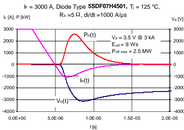
Fig. 6a Snubber diode showing no snap at 1000 A/μs
