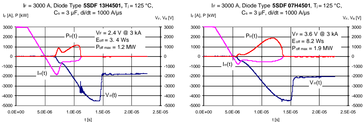
Fig. 5a Uniform life-time FWD, 2.8 kV DC rating
