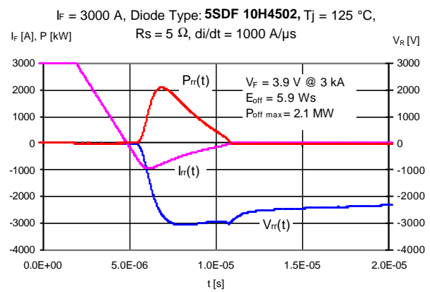
Fig. 6b FWD showing on-set of snap at 1000 A/μs
