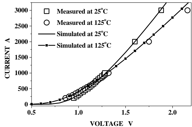
diode at 25 and 125°C
