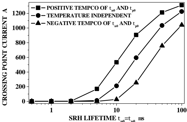
Fig.2: I_{x\text{ing}} vs. lifetime with temperature coefficient \pm 3.4 \times 10^{-4} / \text{K} of t_{n0} and t_{p0} as a parameter
