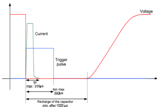
Figure 5. Length of trigger signal to switch
