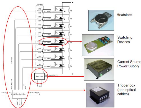
Figure 4. Circuit diagram and assembly main parts
