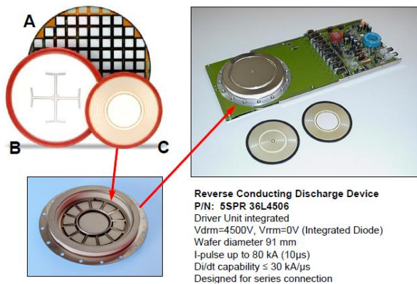
Figure 2. Selection of Silicon Wafers A) IGBT Dies B) Thyristor Wafer C) GCT wafer
