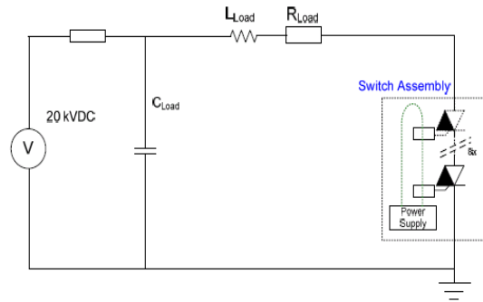
Figure 6. Test circuit of switch assembly
