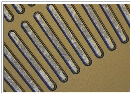
Figure 8. Contact fingers of wafers used in prototype switch after 4 years under application condition use.
