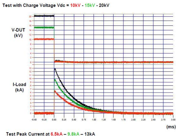
Figure 7. Voltage and Current during pulse test
