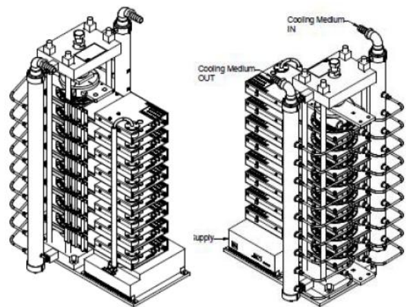
Figure 3. Design Switch Assembly 5SVC083607E03
