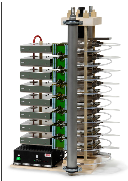
Figure 9. Picture of the complete modulator switch assembly (without triggerbox)
