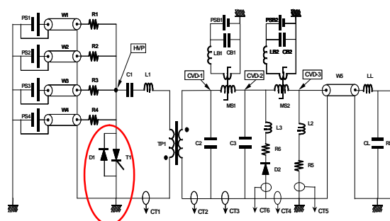
Figure 1. Circuit Diagram Modulator with the reverse conducting solid state switch.
