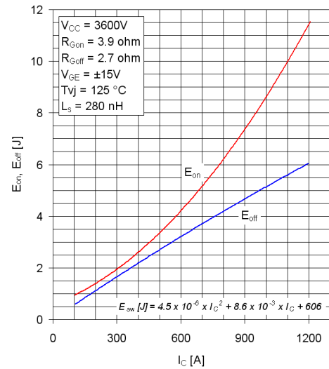
Figure 6. 6.5kV/600A HV-HiPak™ E_{on} and E_{off} vs. I_c losses curves.
