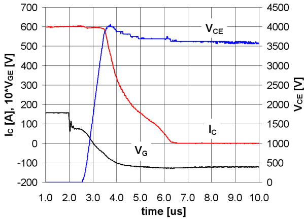
Figure 3. 6500V/600A HV-HiPak™ IGBT nominal turn-off waveforms. V_{CC} = 3600V , I_c = 600A , R_{Gon} = 2.7\Omega , L_\sigma = 300nH , T_j = 125^\circ C .
