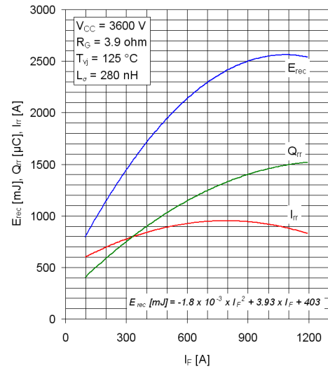
Figure 7. 6.5kV/600A HV-HiPak™ E_{rec} , I_{rr} , Q_{rr} vs. I_F losses curves.
